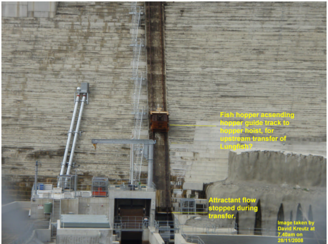
Image 13: Paradise Dam upstream fishway in operation. Fishlift ascending tracks. Taken by David Kreutz on 28 November 2008
